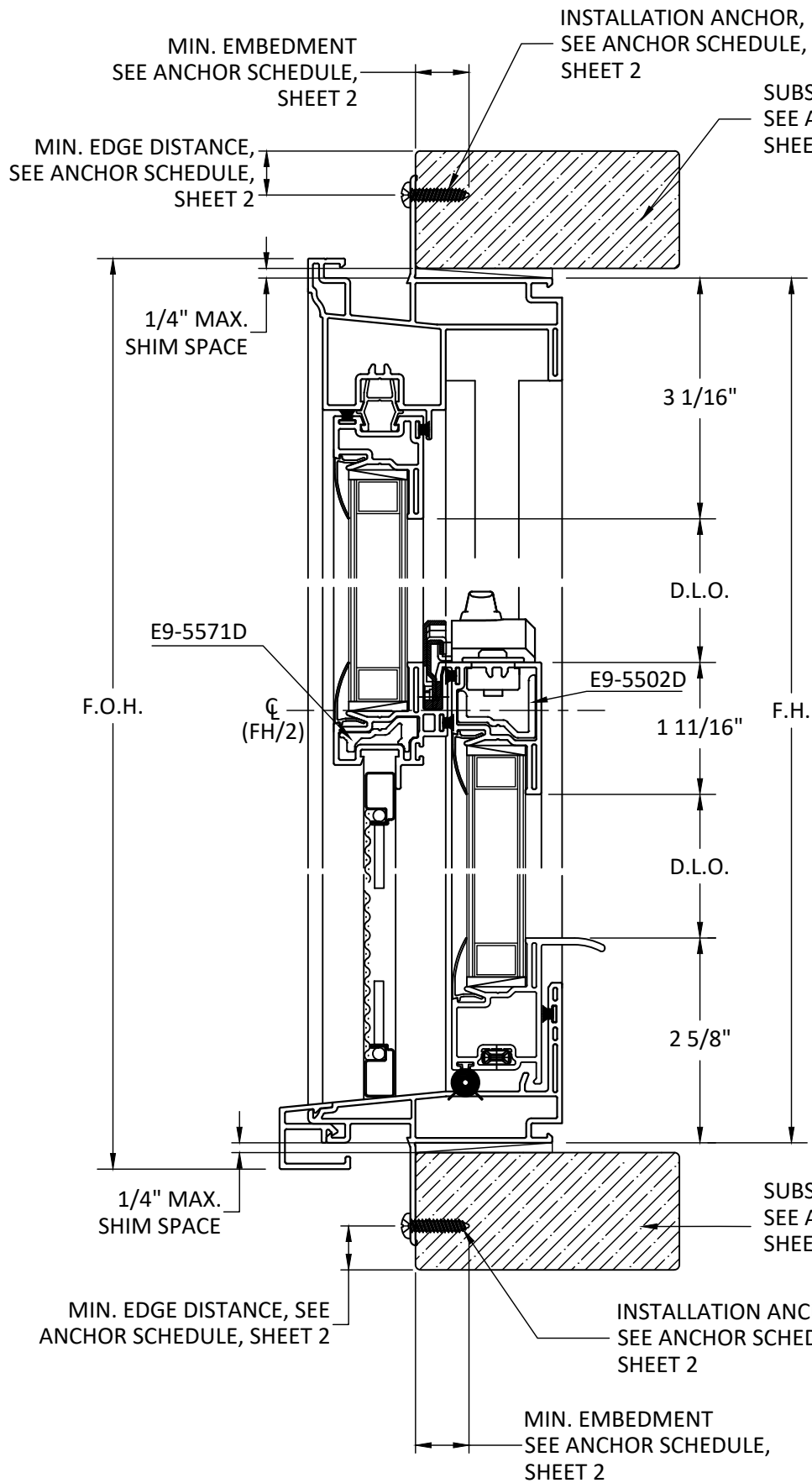
A 3 VERTICAL SECTION FIXED HEAD NAIL FIN
