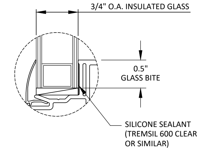
GLAZING DETAIL
