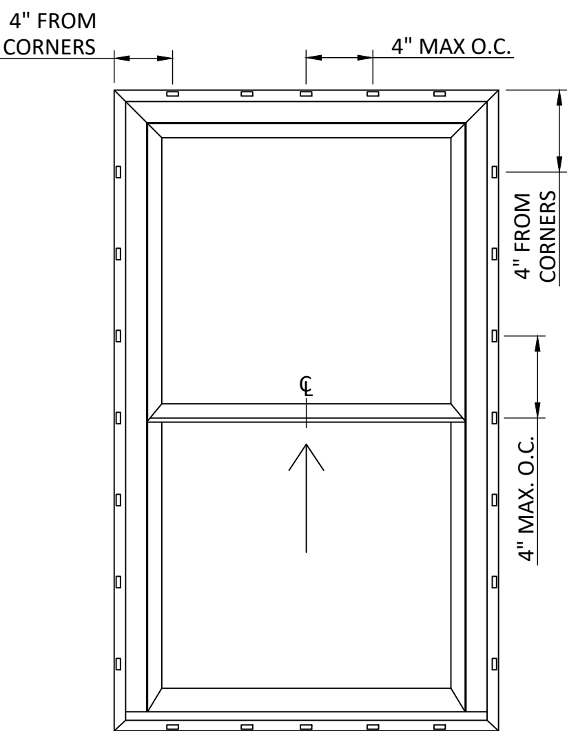
ANCHOR LAYOUT NAIL FIN
